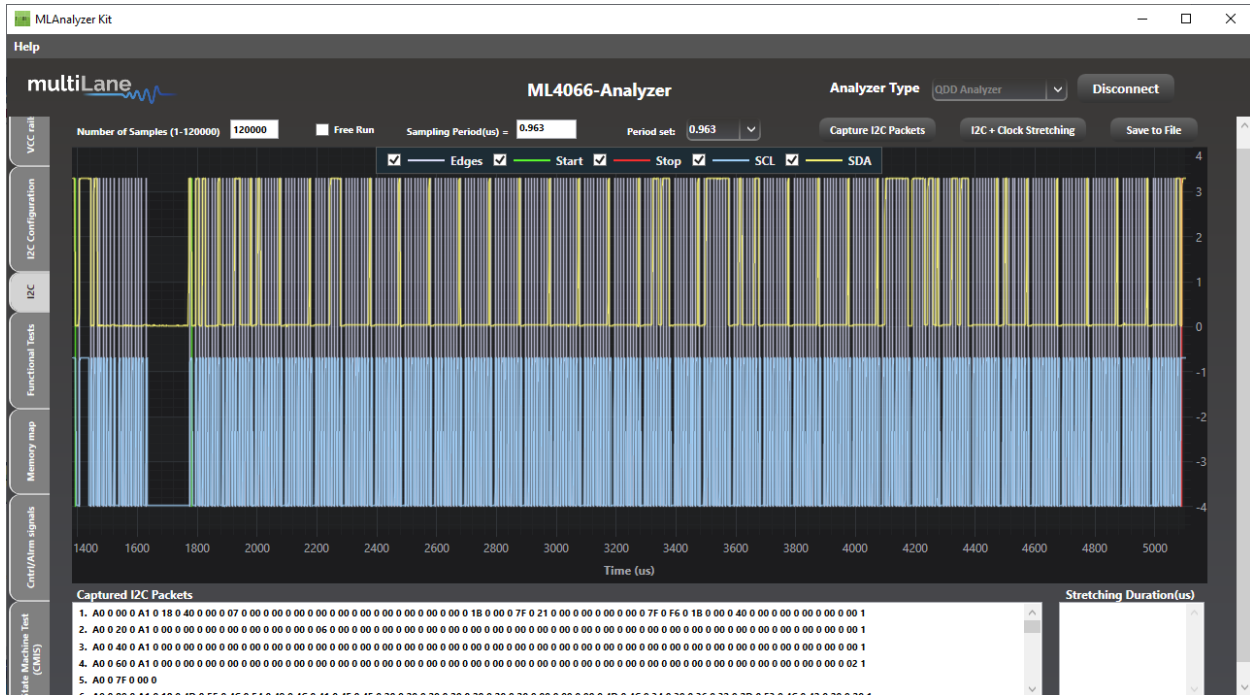
Figure 11: I2C Read
